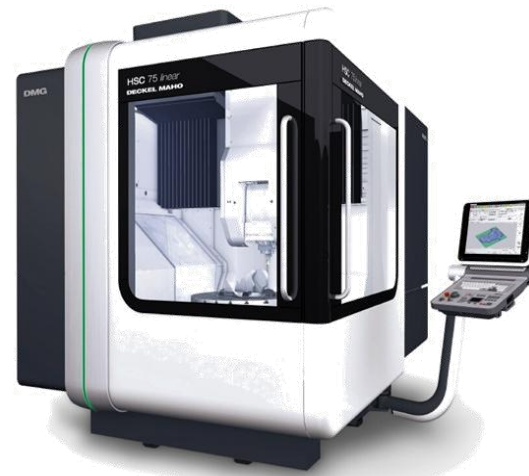
Fig. Milling center for 5-axis simultaneous machining [ISF] .
